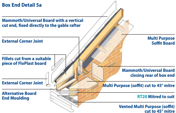
Box End Detail 5a
